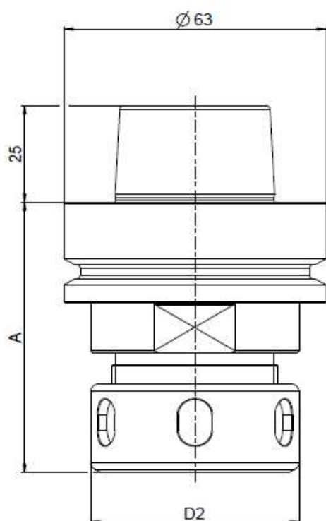
HSK63F
