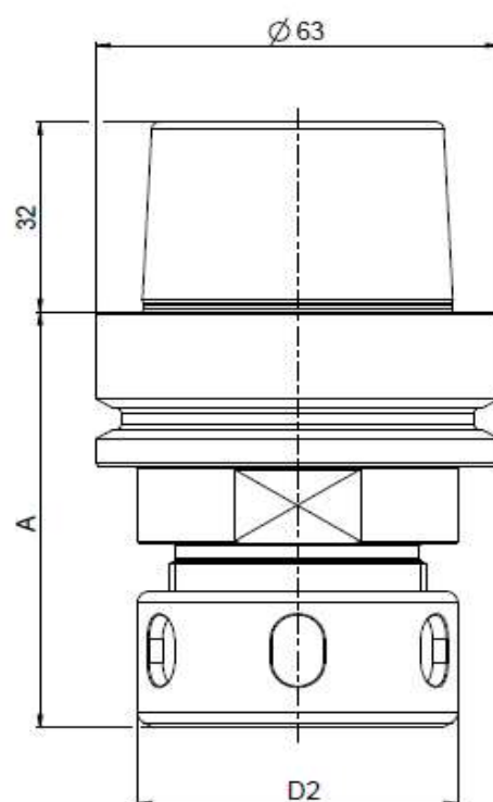
HSK63E
